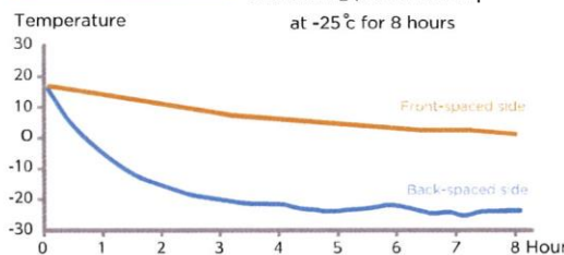
Experimental Temperature Control Data
